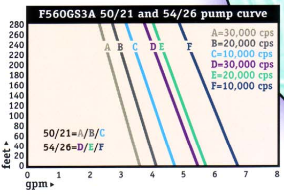
F416 Air Motor and F560GS3A
